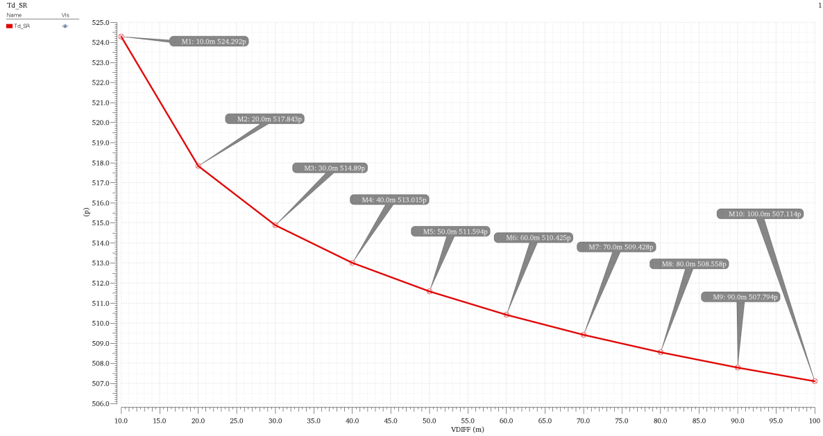
Figure 8: Dynamic slicer delay versus differential input voltage.
