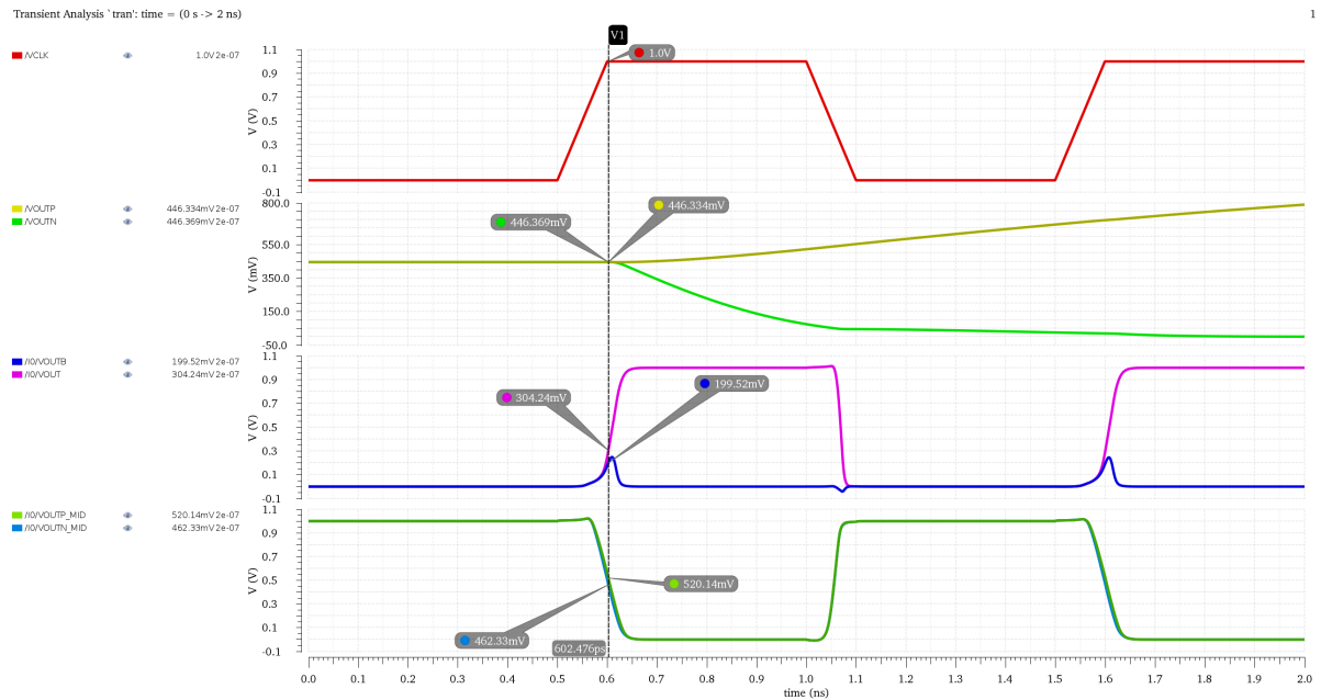
Figure 6: Transient waveforms of the dynamic slicer for PER = 1 ns and VDIFF = 10 mV.
