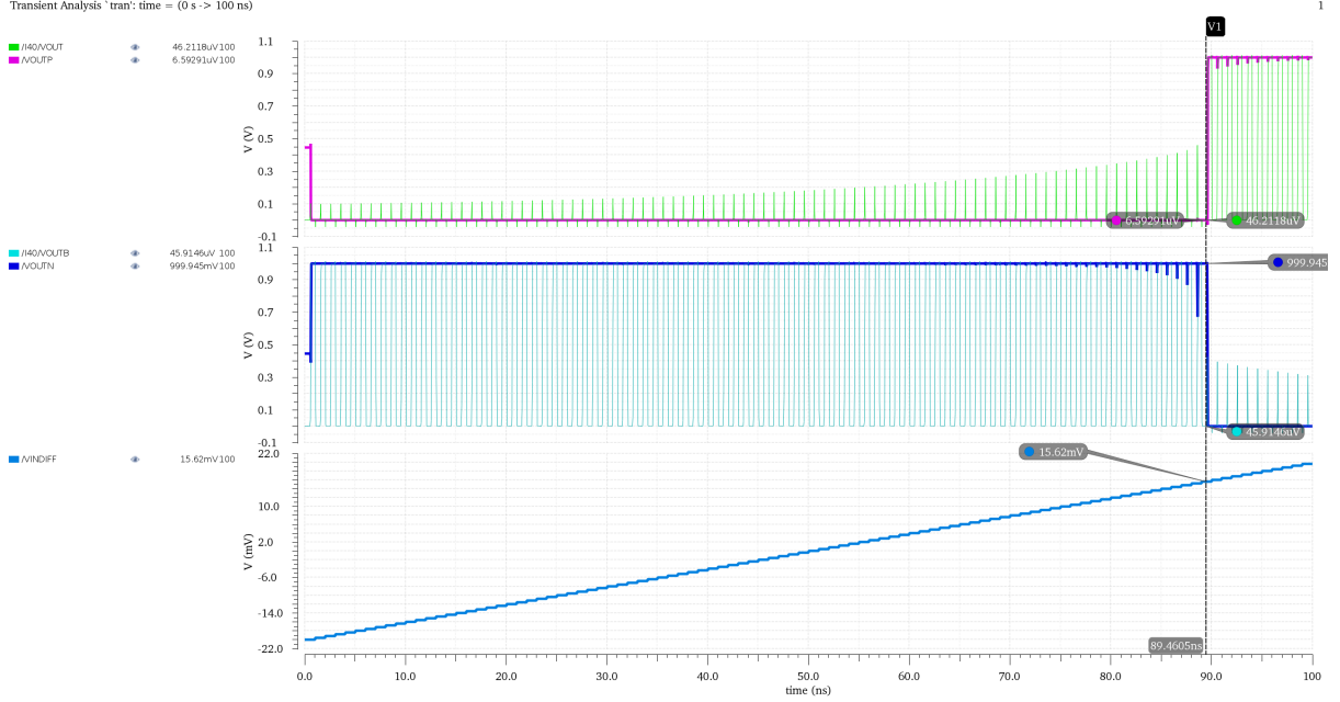
Figure 15: Offset-measurement result and differential-input sweep.
