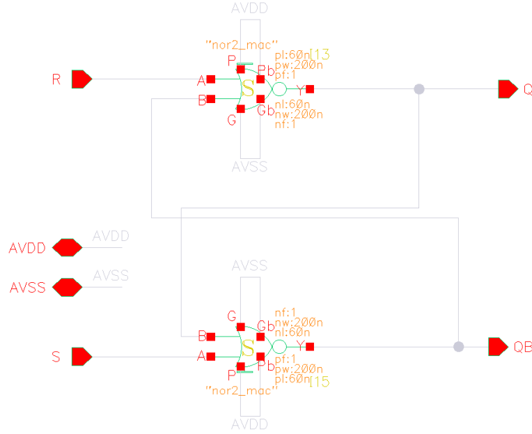
Figure 1: Implemented NOR-based SR latch.
